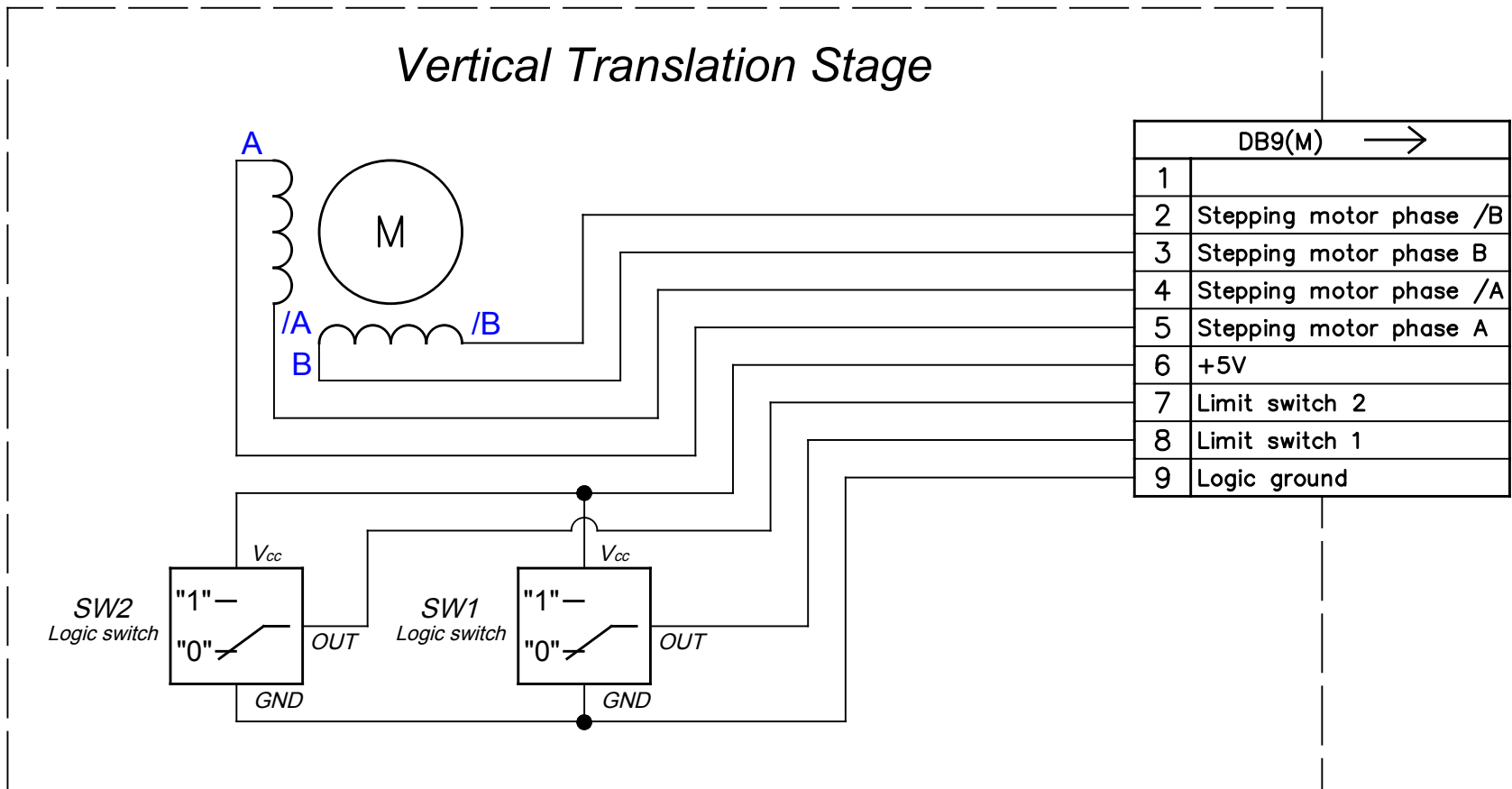
Vertical Translation Stage
