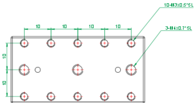
MC#A-2550 (台面尺寸圖)
