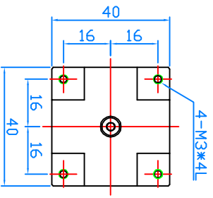
台面鑲嵌板拆除後之上視圖 After floor keysets demolition Top view
