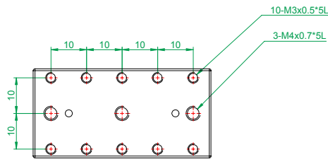
MC#A-2550 (台面尺寸圖)
