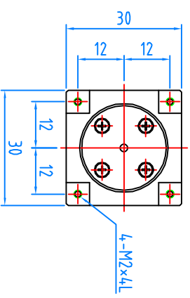
台面轉接板拆除後之上視圖 After floor keysets demolition Top view
