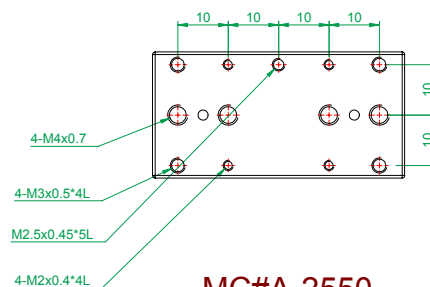
MC#A-2550 (底座尺寸圖)
