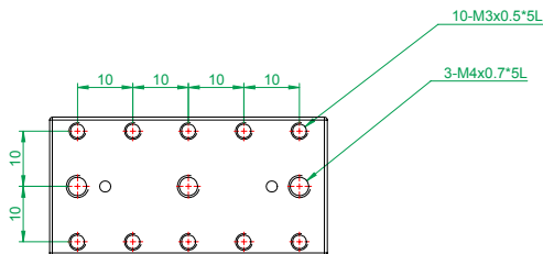
MC#A-2550 (台面尺寸圖)
