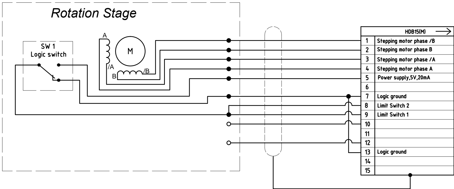
Rotation stage
